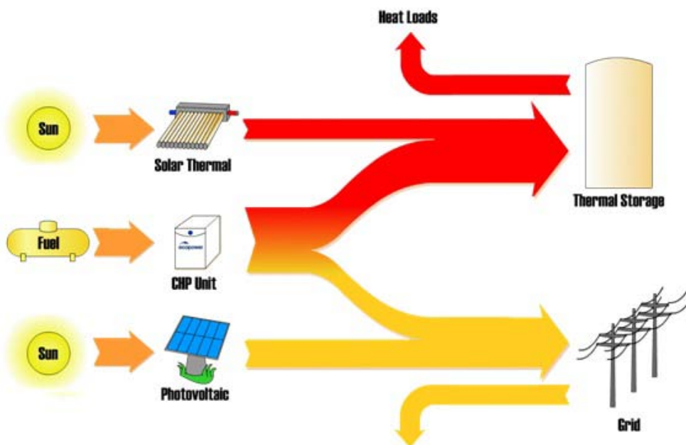
System Overview
